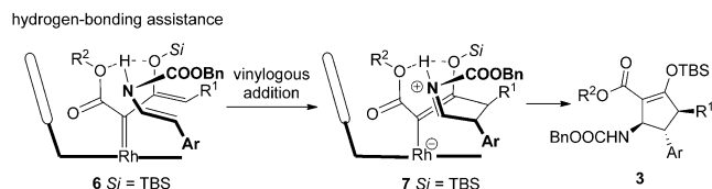
Scheme 4. Proposed mechanism for the [3+2] cycloaddition of an enoldiazoacetate with a trans -enecarbamate.
